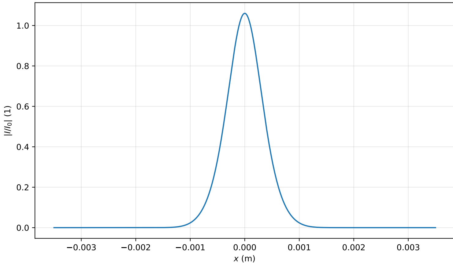
Intensity profile I(x, y = 0, z = 0.796m)/I_0 , P_{in}=0.5P_{cr} , artificial time
